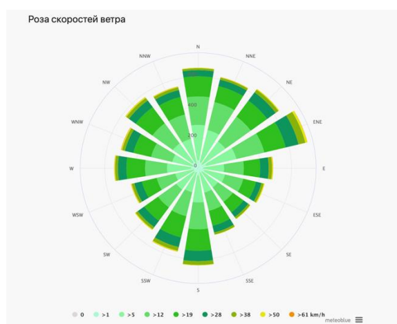
Fig. 2. Wind rose for Kriviy Rih [5].
