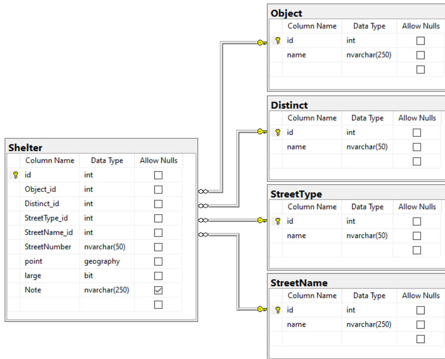
Fig. 1. The general structure of the database
