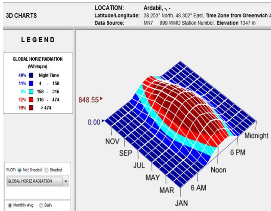
Fig. 4: 3D chart of global horizontal radiation of the sun in the climate of Ardabil city
