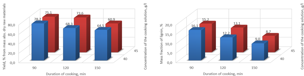
Fig. 2. Dependence of the yield and mass fraction of lignin in the fibrous semi-finished products from Paulownia Clone in Vitro 112 ® wood on the concentration of SO 2 and the duration of cooking at a temperature of 170 °C
