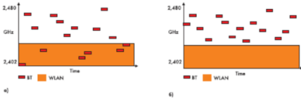
Pic. 2. Principle of operation of AFH technology: a) collisions; b) avoiding collisions using adaptive channel frequency adjustment
