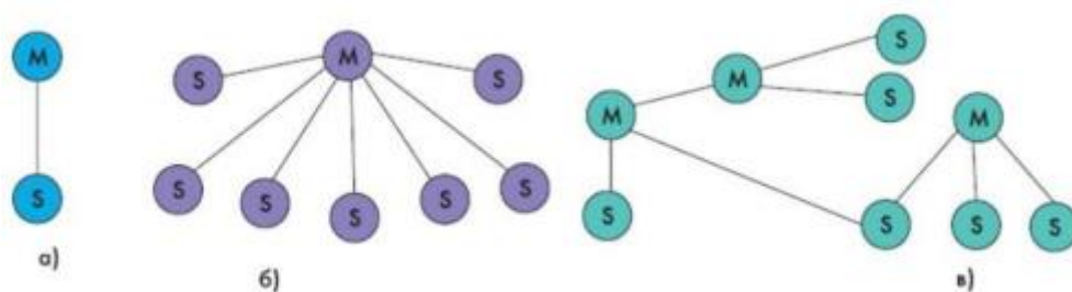
Pic. 1. Pico network with subordinate devices: a) with one subordinate device; b) several; c) distributed network
