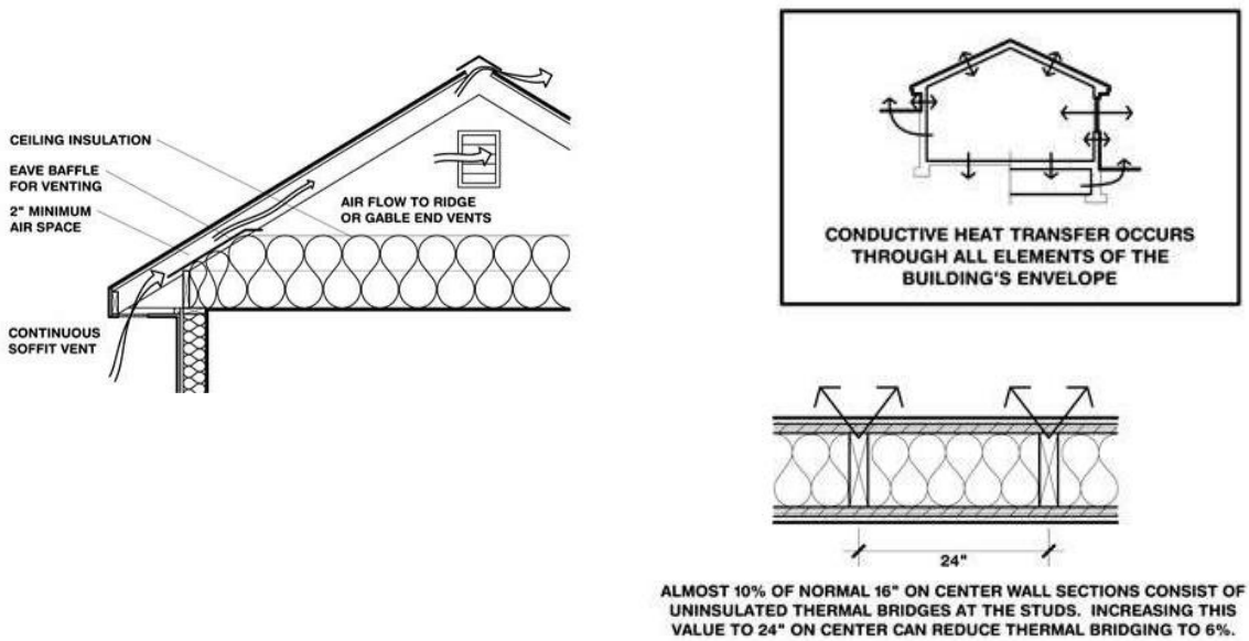
Fig. 5: using high insulation on the outside of the building
