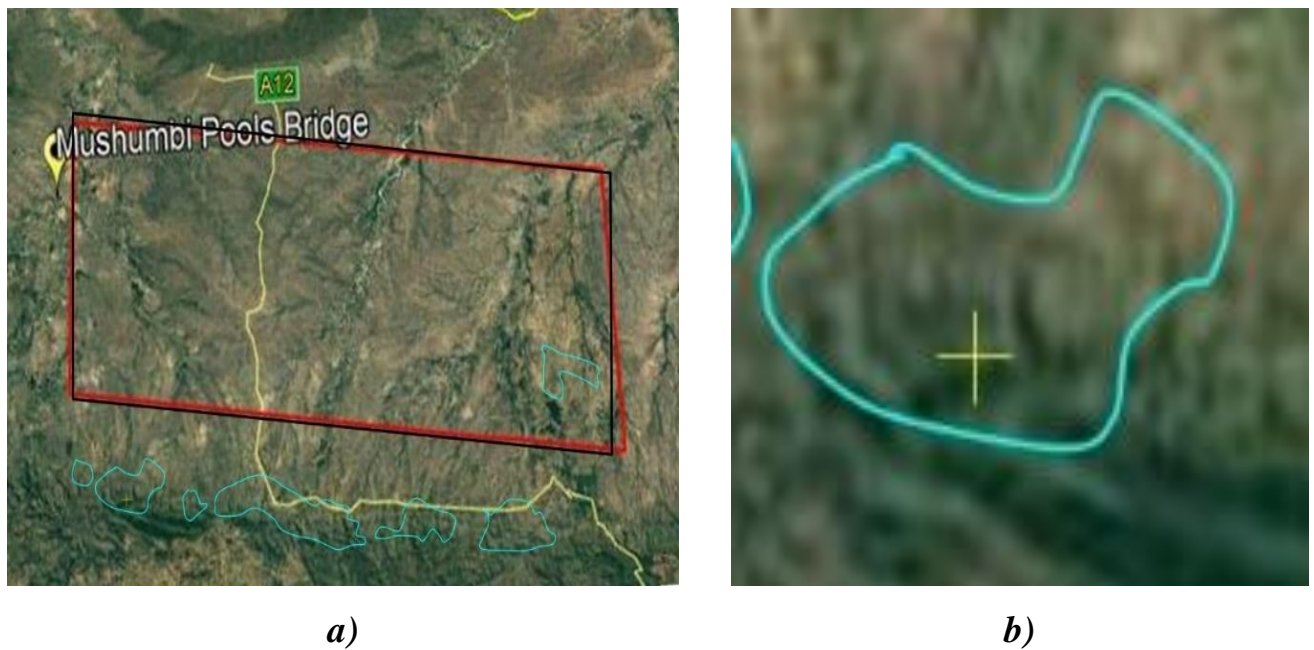
Fig. 5. Position of structural uplifts on the satellite image of the block (a) and image of area of Baobab-1 structure location (b).
