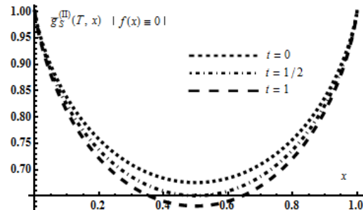
Fig.3. Two particle not normalized distribution function g_S^{(II)}(T, x) without taking into account interaction.
