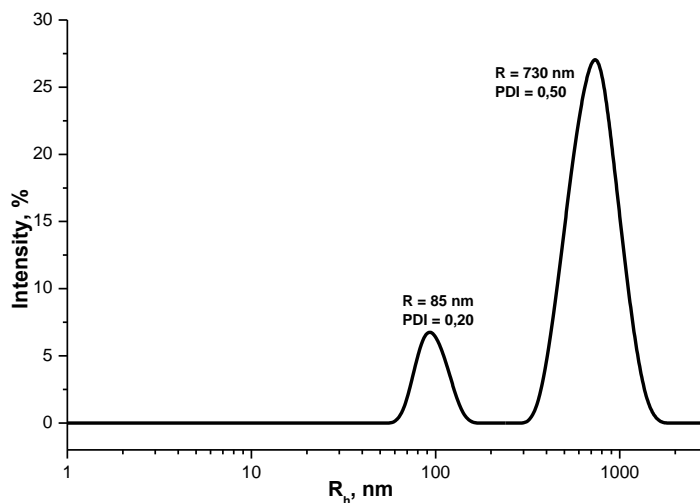
Fig. 2. Hydrodynamic radii of particles of polystyrene dispersion stabilized by lignin-containing polymer
