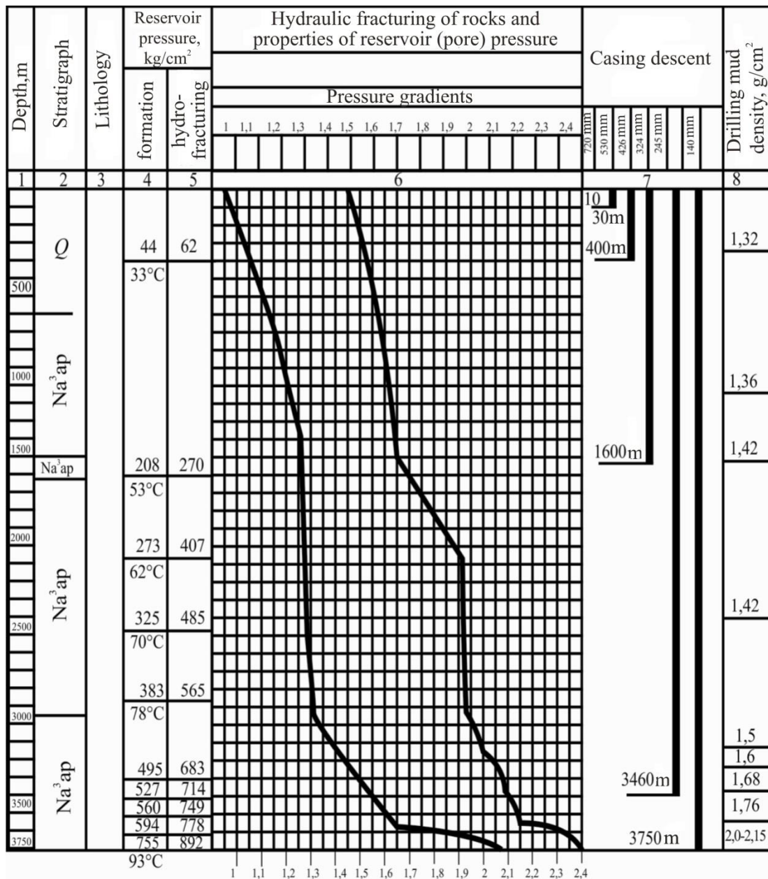
Figure. Combined pressure schedule at the Altgyui field
