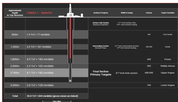
Fig. 3. Illustration of Mukuyu-1 well design [1].
