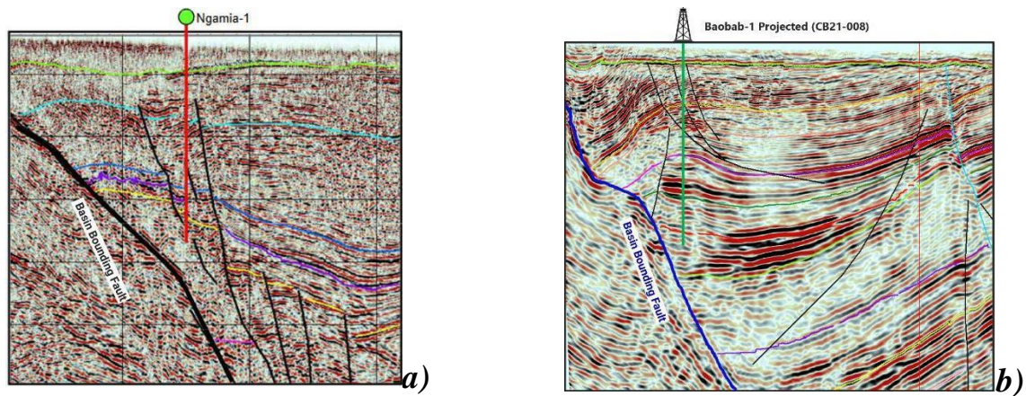
Fig. 6. Ngamia-1 (a) vs. Baobab-1 (b) pre-drill seismic cross-section [1].
