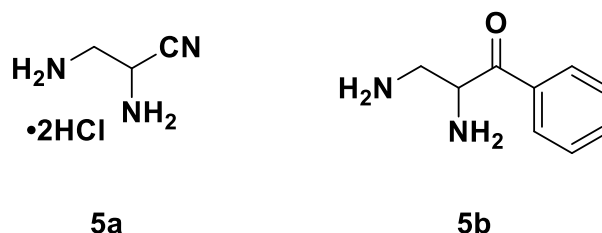
Fig. 1. Structure of the compounds 5a and 5b
