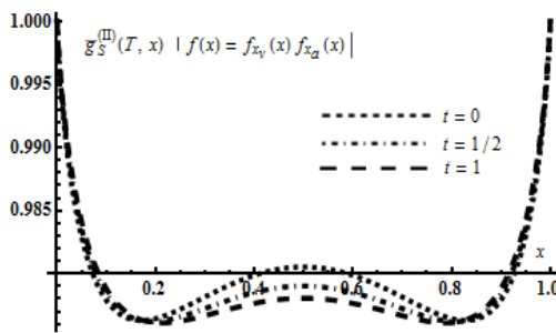
Fig.2. Two particle not normalized distribution function g_S^{(II)}(T, x) with taking into account interaction.
