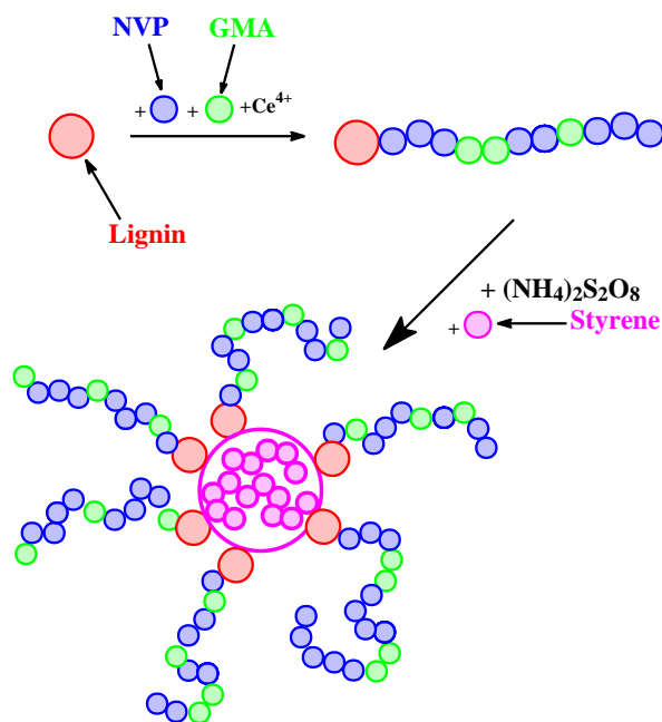
Fig. 1. A two-stage scheme for obtaining a polystyrene dispersion using a lignin-containing polymer as a stabilizer
