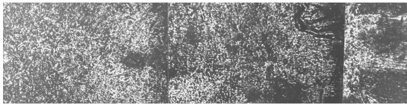
Fig. 4. Microstructure of the base metal (a), transition zone (b) and friction surface (c) of 25XГ2CPΦ steel after quenching and low tempering (I) and quenching and high tempering (II) x500
