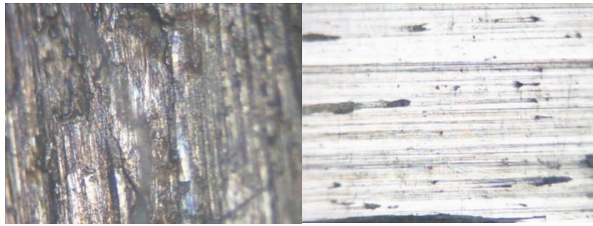
Fig. 3. Condition of the surface of a roller made of steel 25XГ2CPΦ after hardening and high tempering (a) and hardening and low tempering (b) - tests for 60 minutes
