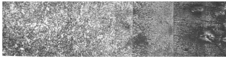
Fig. 3. Condition of the surface of a roller made of steel 25XГ2CPΦ after hardening and high tempering (a) and hardening and low tempering (b) - tests for 60 minutes
