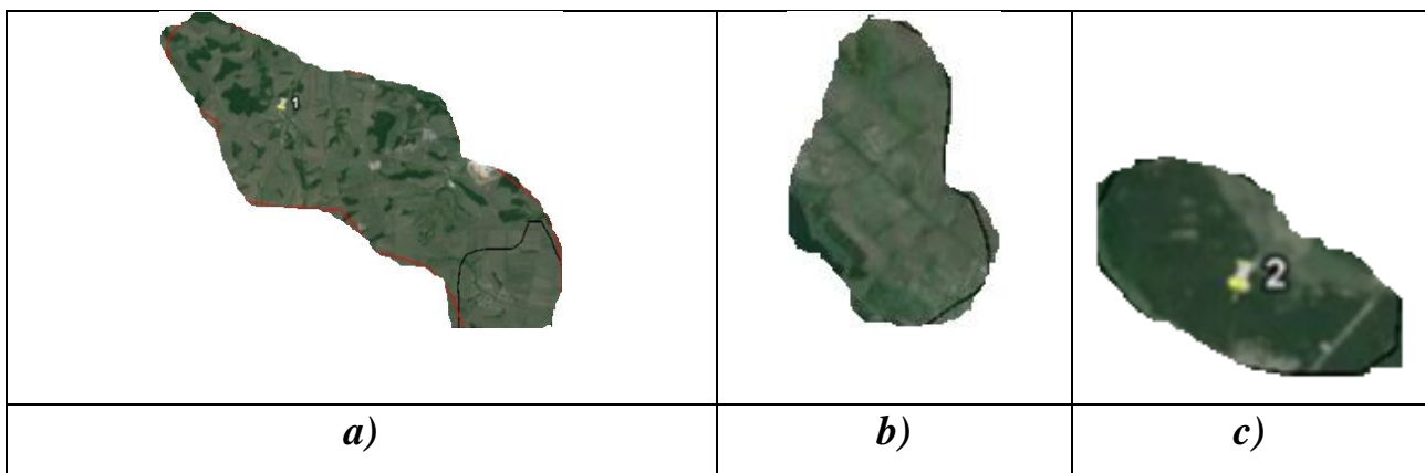
Fig. 2. Satellite images of some blocks in the area of the Shebelynske gas condensate field.
