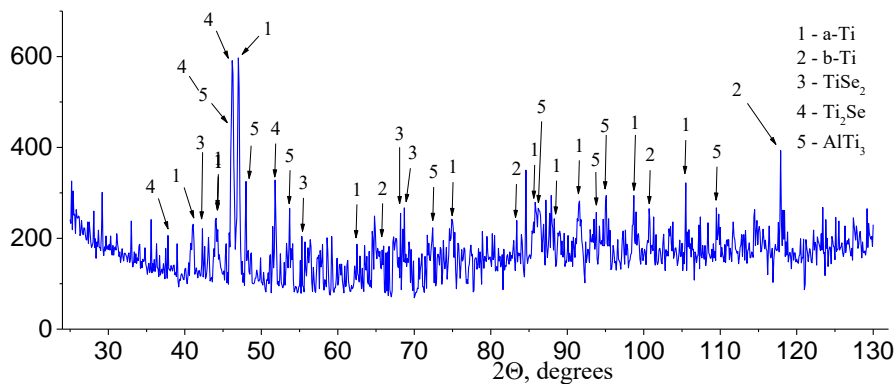
Fig. 2. Diffraction pattern of interaction products in the Ti-Al-Mo+MoSe 2 system during sintering in a vacuum above 1250 °C.
