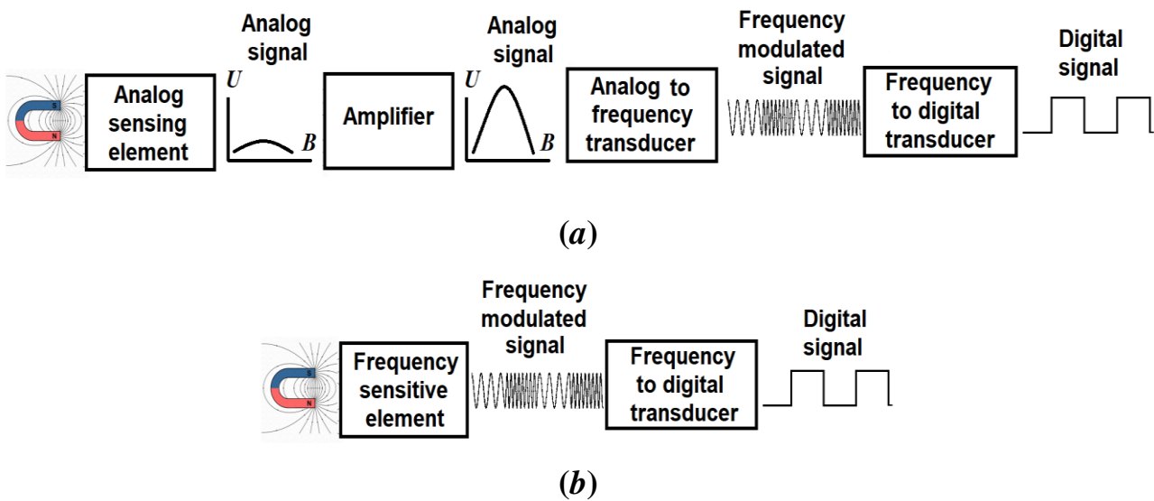
Fig. 1. Comparison of detector components for digital networks based on an analog detector (a) and a detector with a frequency output (b)
