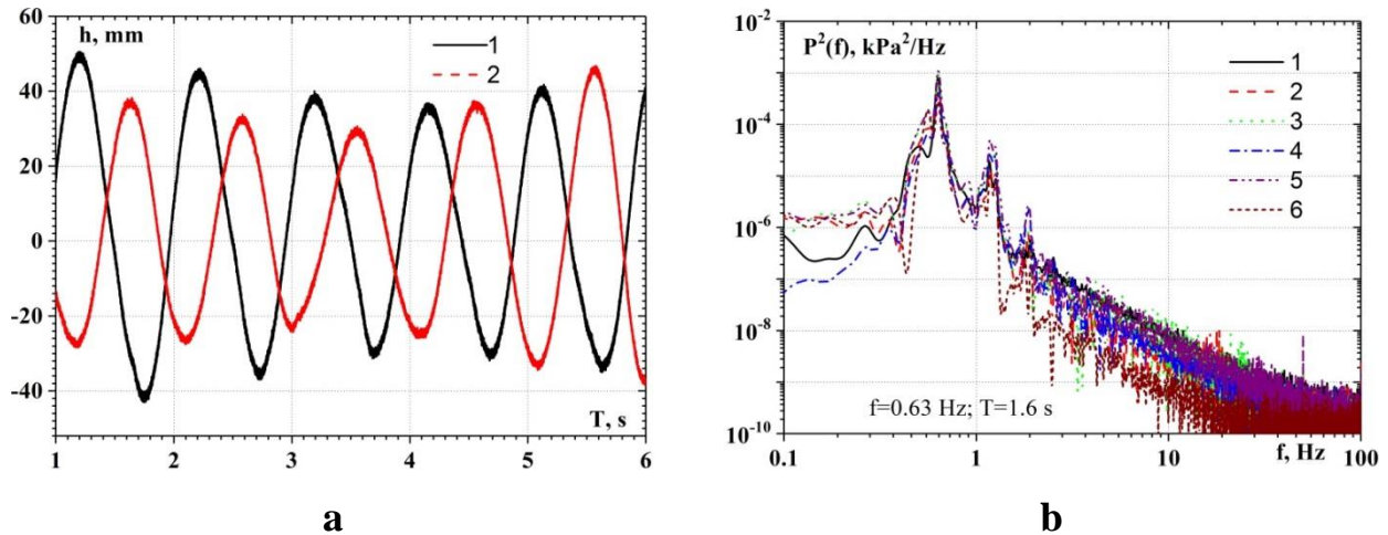
Fig. 3. Shape and height of waves (a) and power spectral densities of wave pressure fluctuations (b) near the permeable wall model
