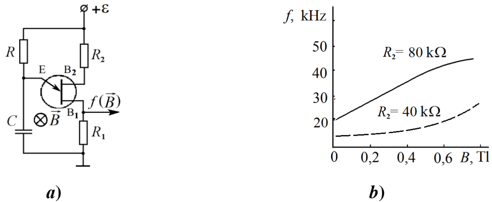
Fig. 3. Scheme of the frequency detector of magnetic field on the UJT (a) and its output characteristics at different values of the limiting resistor (b)
