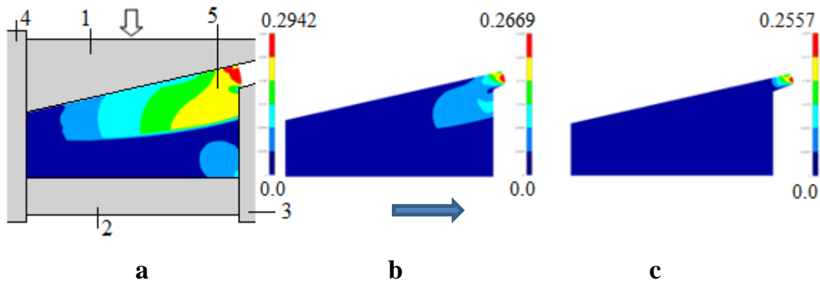
Fig. 1. Forming scheme (a) and porosity distribution at subsequent stamping stages (a, b, c) of a bimetallic blank (1 - upper punch, 2 - lower punch, 3 - matrix, 4 - mandrel, 5 - blank; initial porosity of the upper layer 0.3, the lower one - 0.15)
