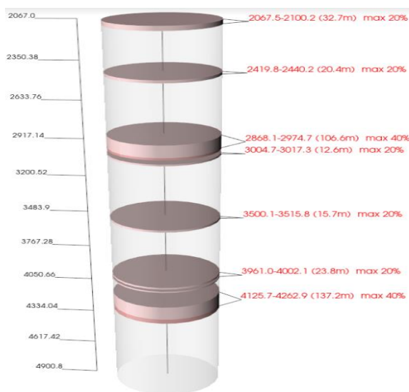
Fig. 8. Anomalous zone Shirokovskaya: results of scanning with a 10 cm step.
