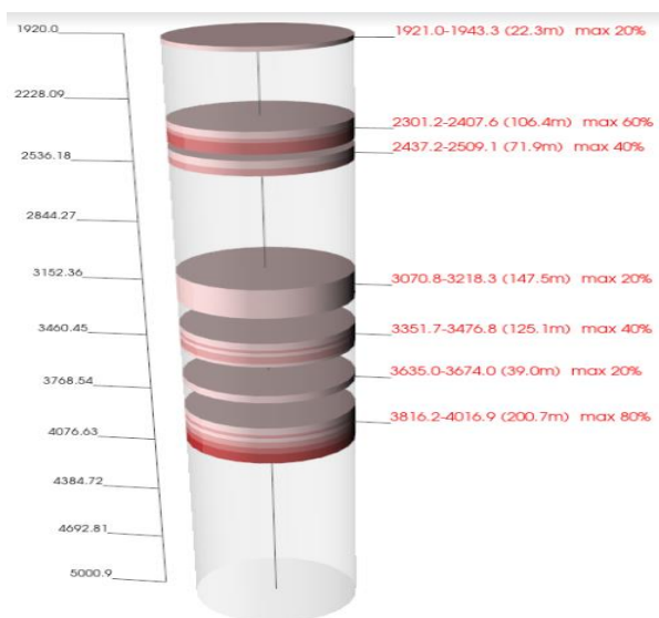
Fig. 6. Anomalous zone Alekseevskaya: results of scanning with a 10 cm step.
