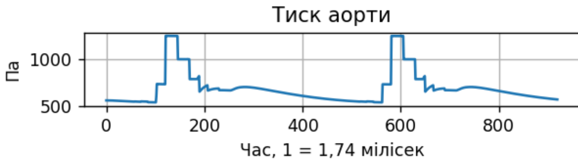
Fig. 10. Time dependence of the pressure of an arterial vessel
