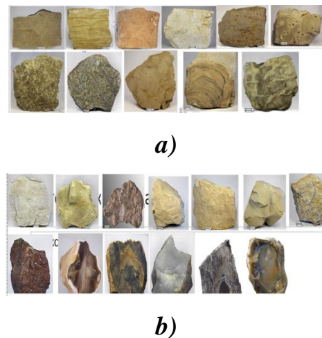
Fig. 3. Photos of the 8th (dolomite) (a) and 10th (siliceous) (b) groups of sedimentary rocks.
