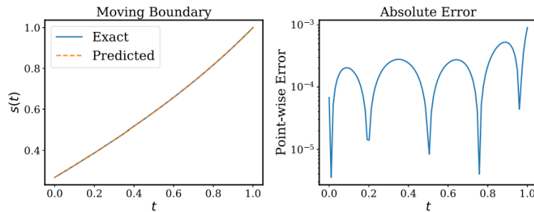
Fig. 2 Direct one-dimensional one-phase Stefan problem
