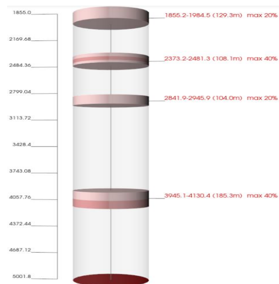
Fig. 9. Anomalous zone Sergeevskaya: results of scanning with a 10 cm step.
