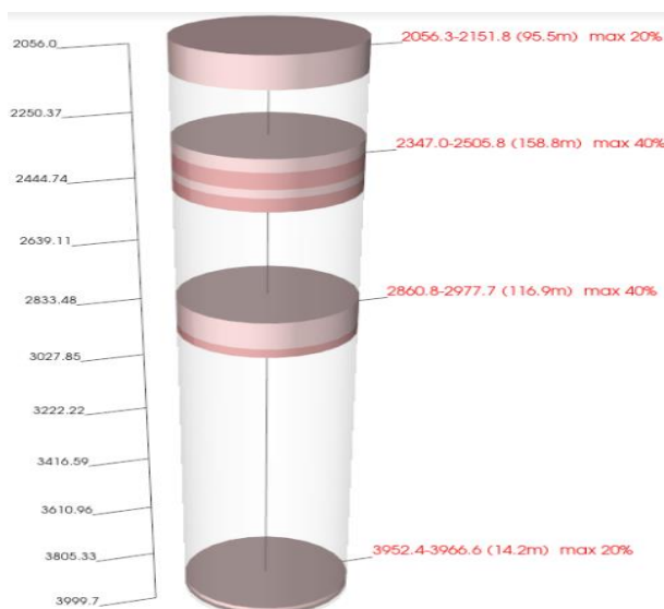
Fig. 7. Anomalous zone Shabovskaya: results of scanning with a 10 cm step.
