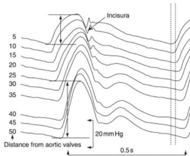
Fig. 14. Literary experimental data on the dependence of pressure in the human aorta depending on the distance from the heart and the direction of the aorta relative to the Earth's gravity field direction.
