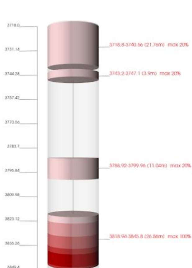
Fig. 5. Graphic representation of the results of the cross-section scanning in the depth range of 3500-4000 m.
