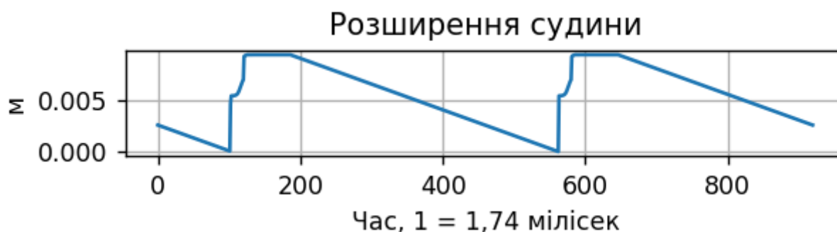
Fig. 5. Time dependence of the degree of expansion and narrowing of the arterial vessel
