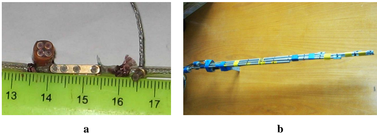
Fig. 2. Piezoceramic pressure fluctuation sensors (a) and piezoresistive wave height sensors (b)
