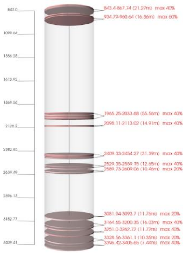
Fig. 4. Graphic representation of the results of the cross-section scanning in the depth range of 0.8-3500 m.
