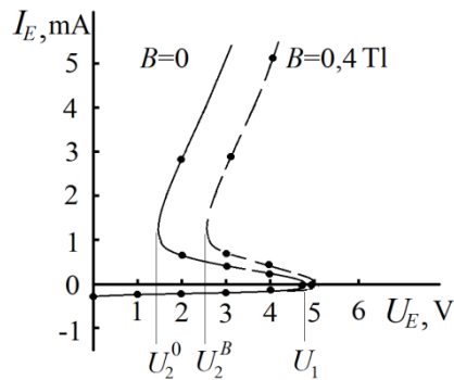
Fig. 2. Current-voltage characteristic of UJT without and during the action of a magnetic field
