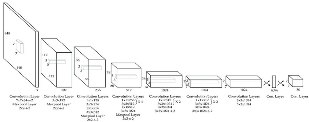
Fig. 1. Architecture of the YOLO model for a 448 by 448 image.
