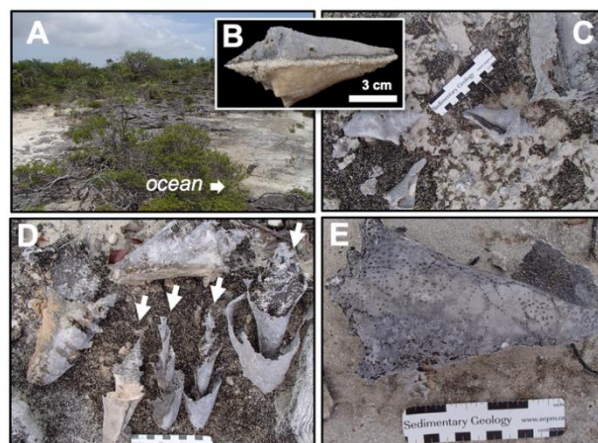
Figure 2. Aliger gigas shells: A) Paleoshoreline I (see Fig. 1 for location); B) This shell is nearly unaltered below the sediment surface and highly corroded (gray) above it; C) Examples of different fragmentation patterns; D) relatively well preserved shells (top) and columellas (arrows); E) Extensive sponge borings ( Entobia isp. ) permeate this shell.
