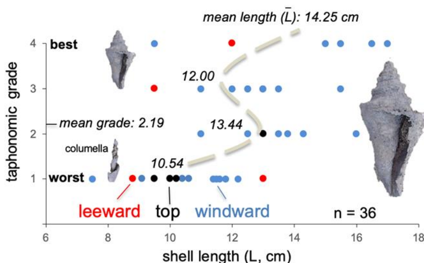
Figure 3. Taphonomy: nearly half (39%) of specimens show poor preservation (grade 1), with a general improvement with specimen size.
