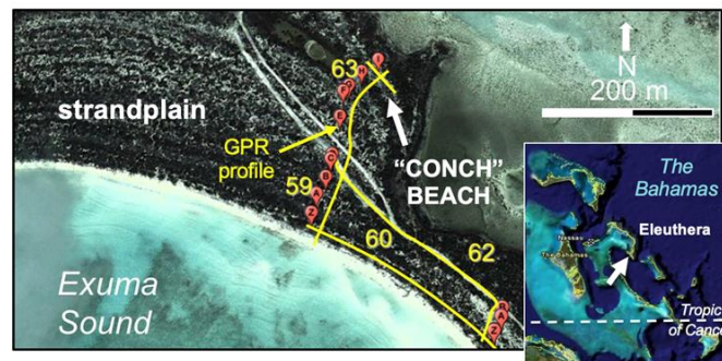
Figure 1. The study site is a Holocene strandplain along the southern Eleuthera Island, The Bahamas (see arrow in the inset for location within the archipelago).
