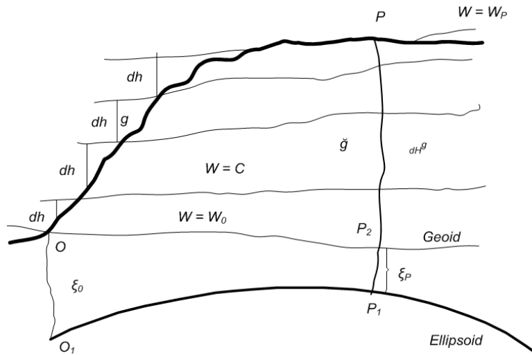
Fig. 1. Orthometric excesses and height of the geoid
