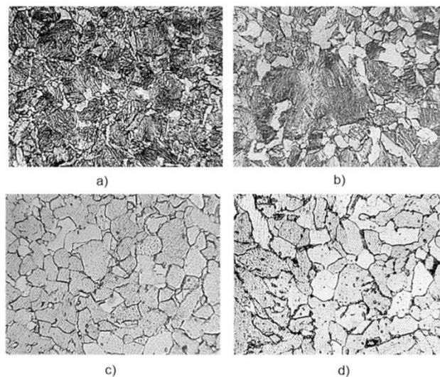
Fig. 2 Microstructure of steel samples St1kp (modification) x500, cooling rates, quenching temperatures a) - V_{cool}=3.60C/s t_{QUIENING} = 795^0C ; b) - V_{cool}=3.60C/s t_{HARDENING} =700^0C ; c) - V_{cool}=3.60C/s t_{QUIENING} = 670^0C ; d) - V_{cool} = 3.60 C/s t_{QUICKENING} = 570^0 C
