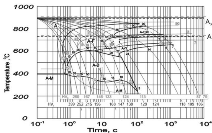
Fig. 1 Thermokinetic diagram of austenite decomposition of modified and serial steel St1kp
