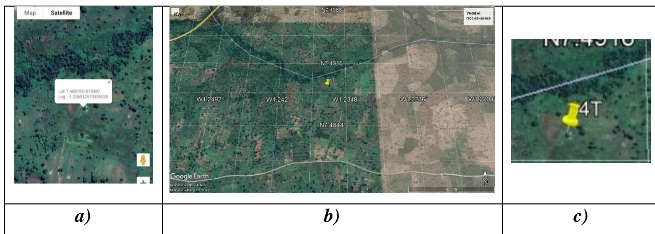
Fig. 1. Satellite images of a different fragments of the territory within the survey area.
