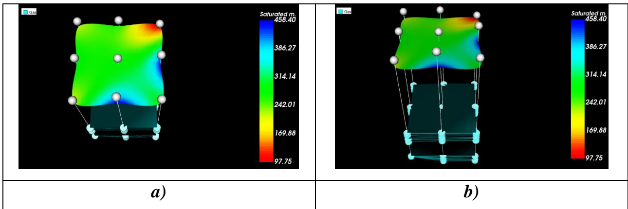
Fig. 4. Three-dimensional graphical images of the results of scanning the cross-section at 9 points.
