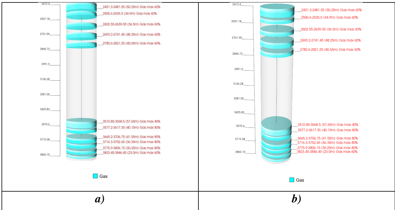
Fig. 3. Visualization of scanning results at one point of the site in 2 formats.
