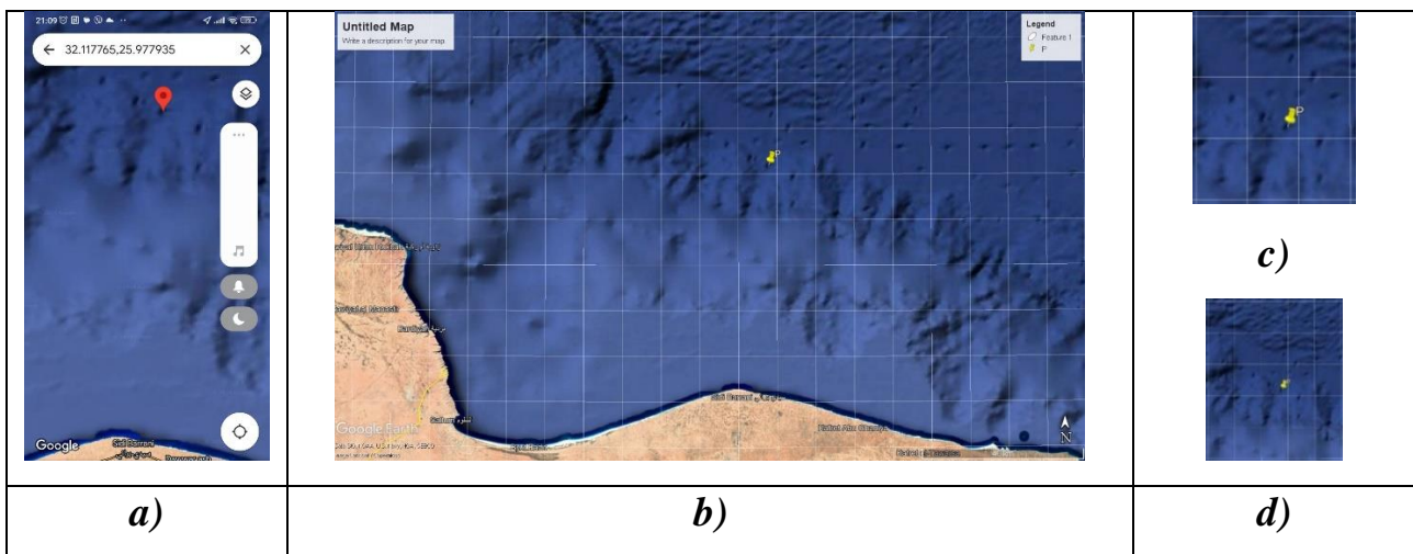
Fig. 1. Satellite images of study area in Mediterranean Sea with point coordinates (a) and prepared for frequency-resonance processing in “Google Earth” software package (b, c, d).
