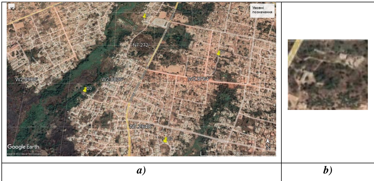
Fig. 2. Satellite image of Dormaa area (a) and a fragment of territory within the demo site (b). (The fragment is larger than 100*100 m).
