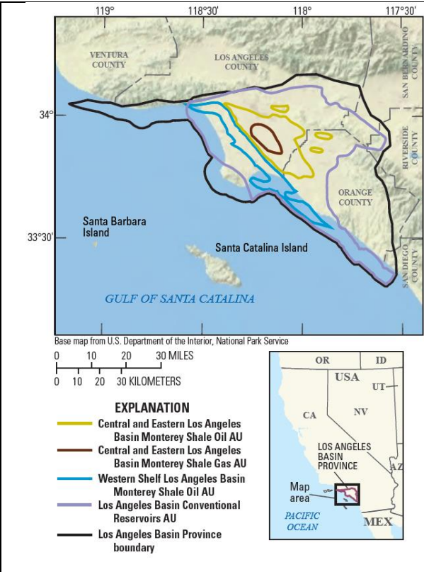
Fig. 1. Maps showing location of four assessment units (AUs) in the Los Angeles Basin Province [8].
